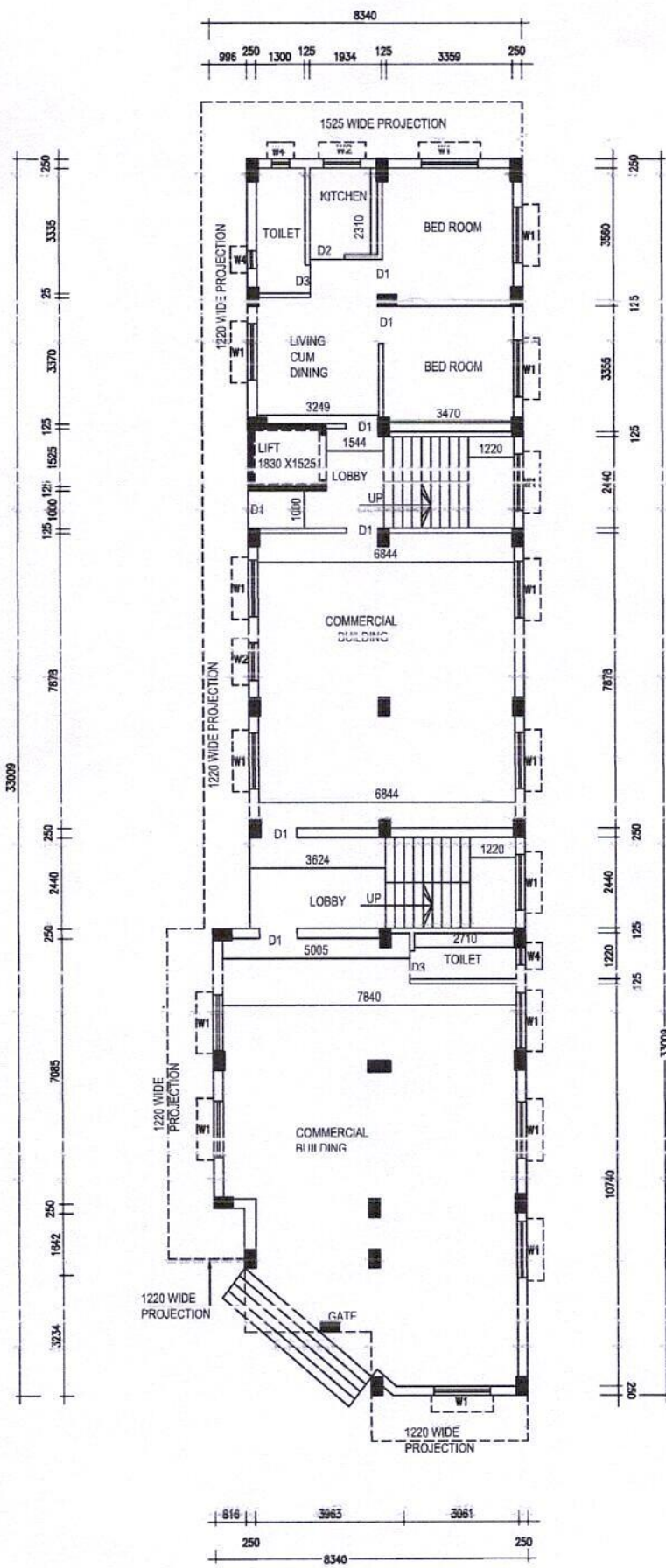
GROUND FLOOR PLAN (SCALE=1:100)
